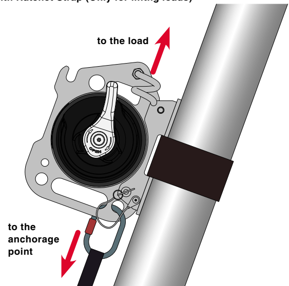
Fixing with Ratchet Strap (Only for lifting loads)
